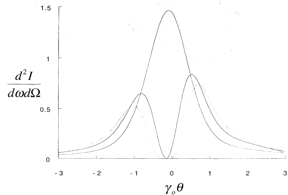
FIG. 5. Circular polarization, transverse scattering. Normalized intensity of the first three harmonics of Fig. 4 along the x' axis of the detector, a_0=2 , \gamma_0=10 . Distance along the axis is measured in units of \gamma_0(x'/z'_0) \sim \gamma_0\theta .
