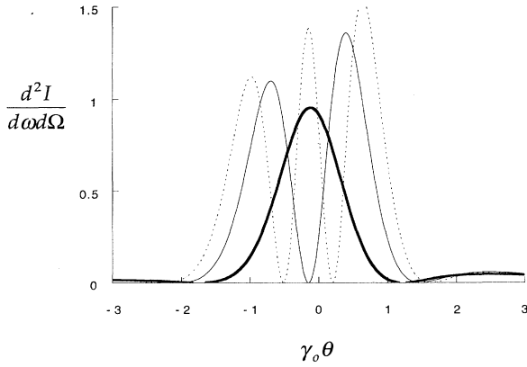
FIG. 10. Linear polarization, transverse scattering, \beta_{1y} = 0 . Normalized intensity of the first three harmonics of Fig. 9 along the x' axis of the detector. Distance along the axis is measured in units of \gamma_0(x'/z'_0) \sim \gamma_0\theta .
